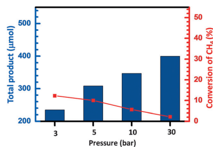
Figure 3. Pressure-dependent catalytic performance in partial oxidation of \text{CH}_4 on 0.01 wt % Pd/ZSM-5 at 95^\circ\text{C} . 28 mg of catalyst, 0.01 wt % Pd/ZSM-5 was added to a Parr reactor; 10 mL de-ionized \text{H}_2\text{O} was added; \text{H}_2\text{O}_2 (5 mmol) was added to \text{H}_2\text{O} before \text{CH}_4 was introduced to the Parr reactor. The plotted yield of a product formed on 28 mg 0.01 wt % Pd/ZSM-5 is the value after subtraction of the yield of the products formed on 28 mg ZSM-5 (without Pd sites) under the same catalytic conditions.
