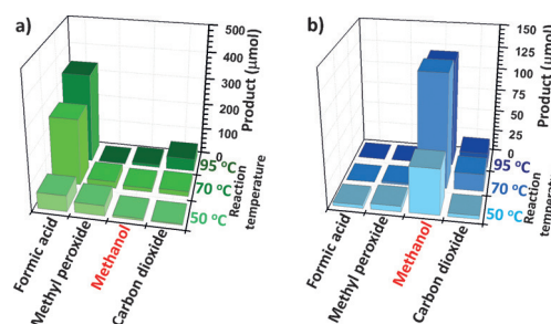
Figure 4. Catalytic performance of a) 0.01 wt % Pd/ZSM-5 at 50, 70, and 95^\circ\text{C} , and b) 0.01 wt % Pd/ZSM-5 loaded with 2 wt % CuO at 50, 70, and 95^\circ\text{C} . The plotted yields of products formed on 28 mg 0.01 wt % Pd/ZSM-5 or 0.01 wt % Pd/ZSM-5 loaded with 2.0 wt % CuO are the values after subtraction of the yields of the products formed on 28 mg ZSM-5 (without Pd sites) under the same catalytic conditions.
